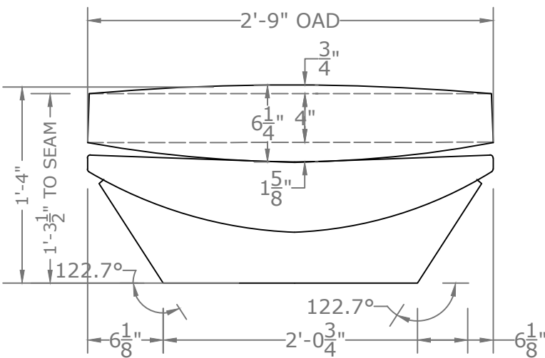
B SECTION B - B - OTTOMAN NTS
