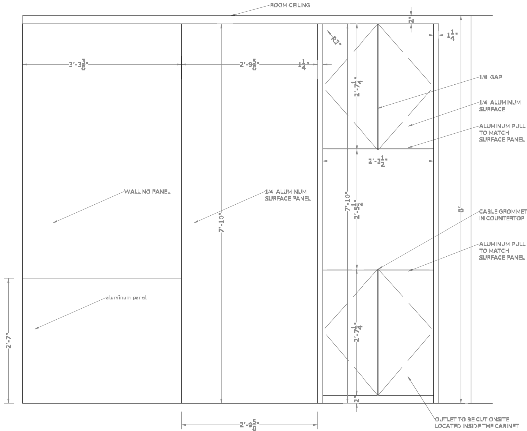
M SHELF FRONT AND PANEL VIEW NTS
