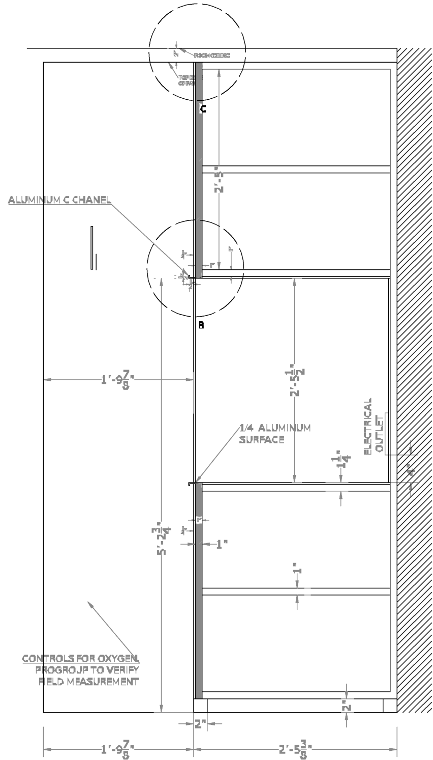
L SHELF SECTION G - G NTS
