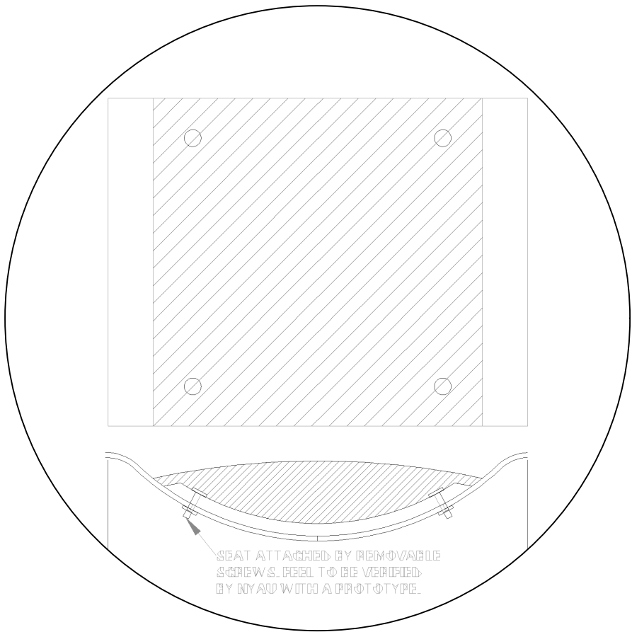
S DETAIL E - REMOVABLE CUSHION SEAT ATTACHMENT TO SEAT NTS
