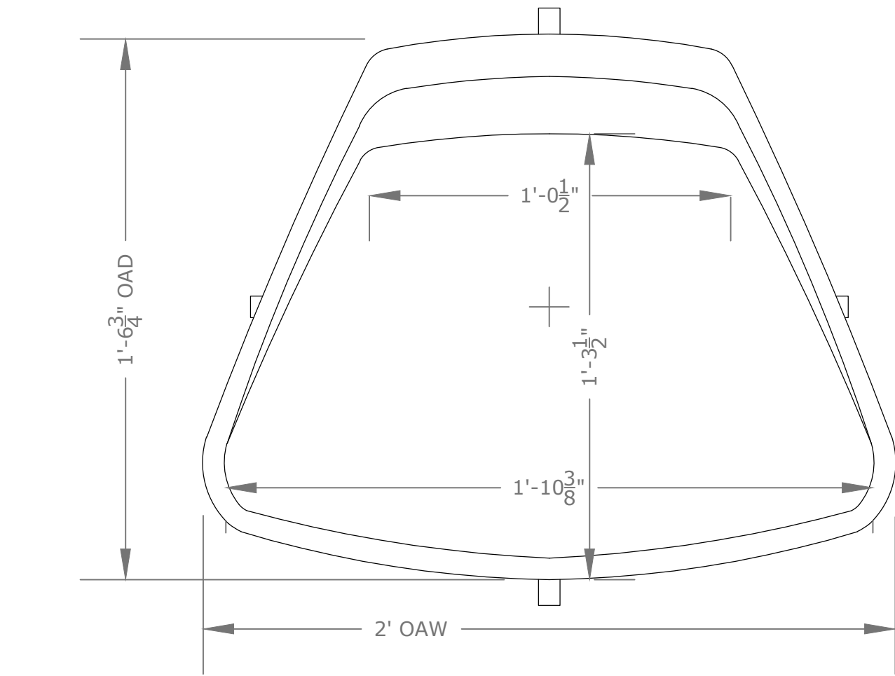
A PLAN VIEW NTS
