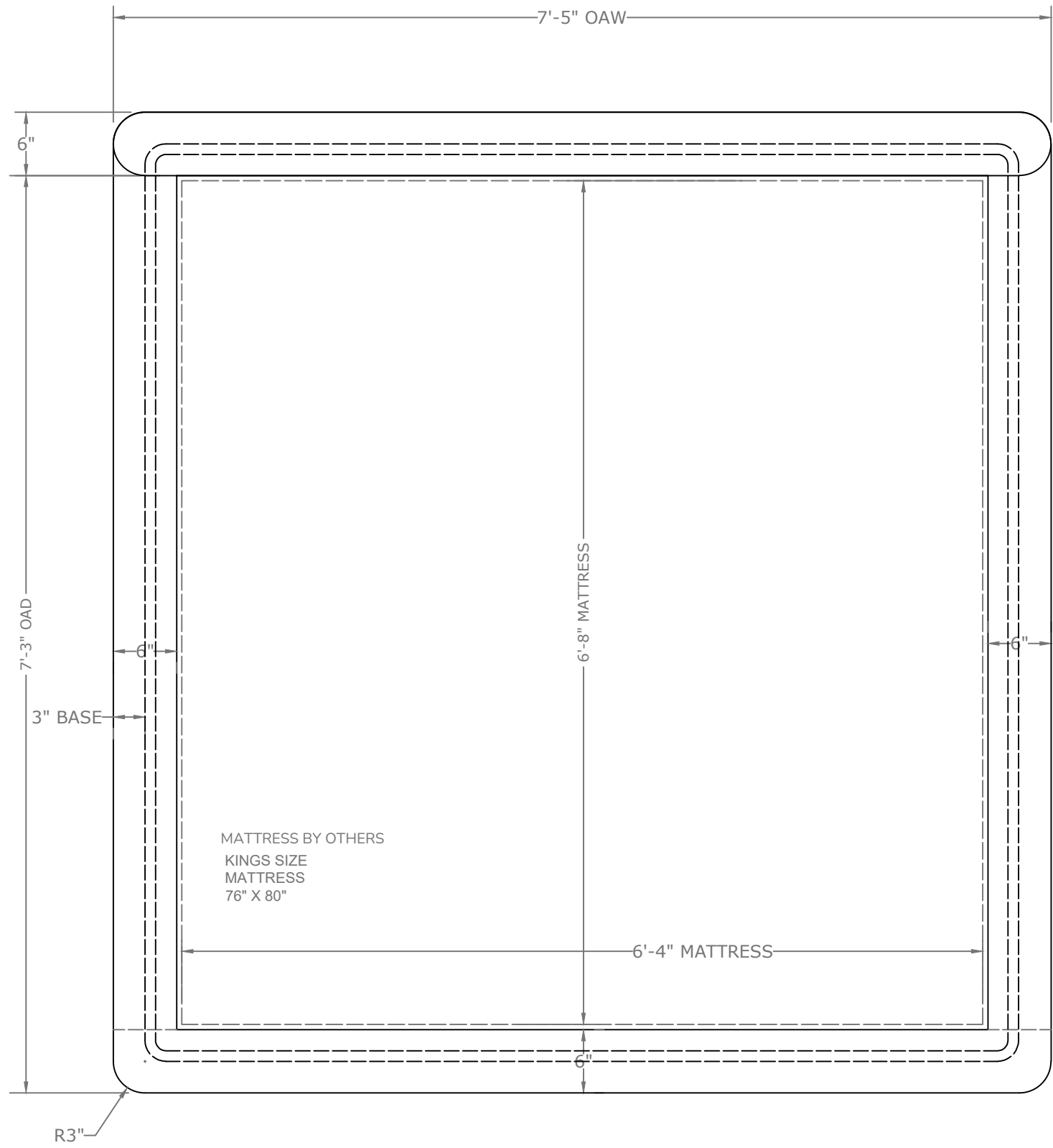
A PLAN VIEW NTS
