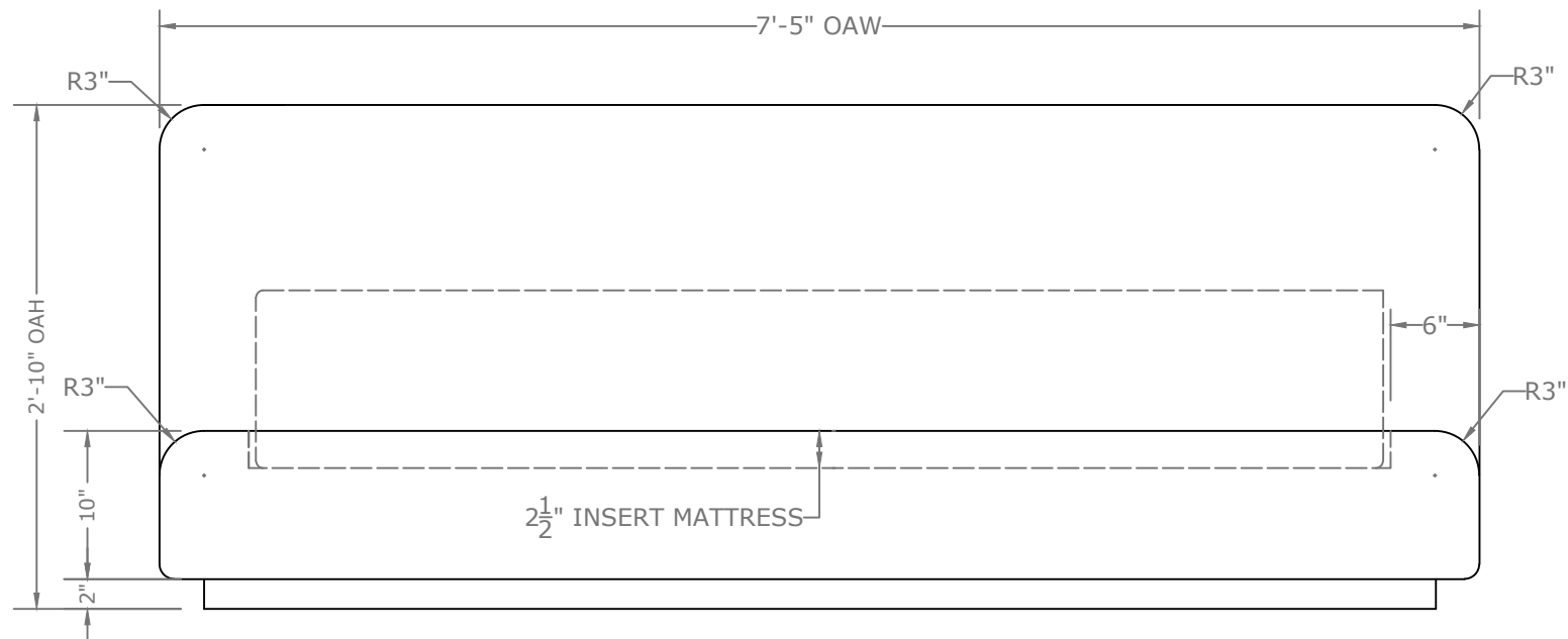
B FRONT VIEW NTS
