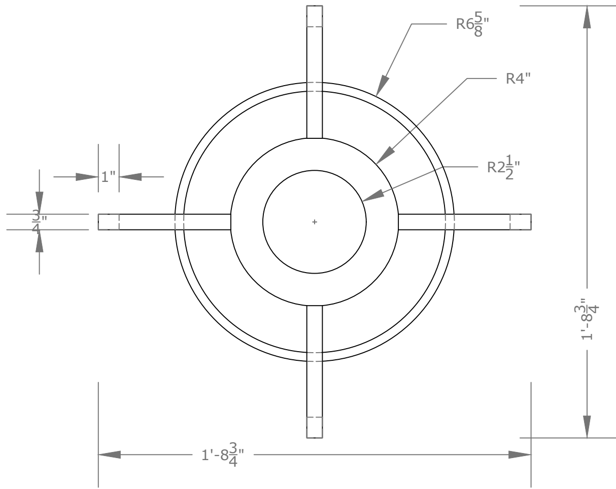
D PLAN VIEW - LEGS NTS
