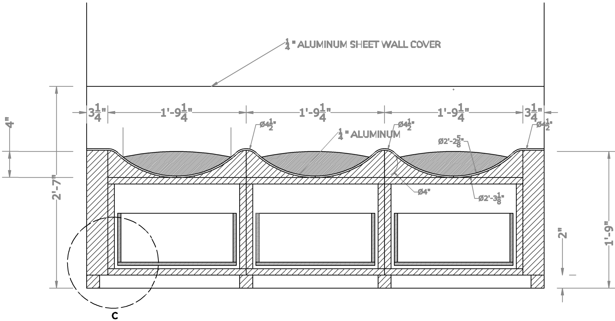
C SECTION C - C NTS
