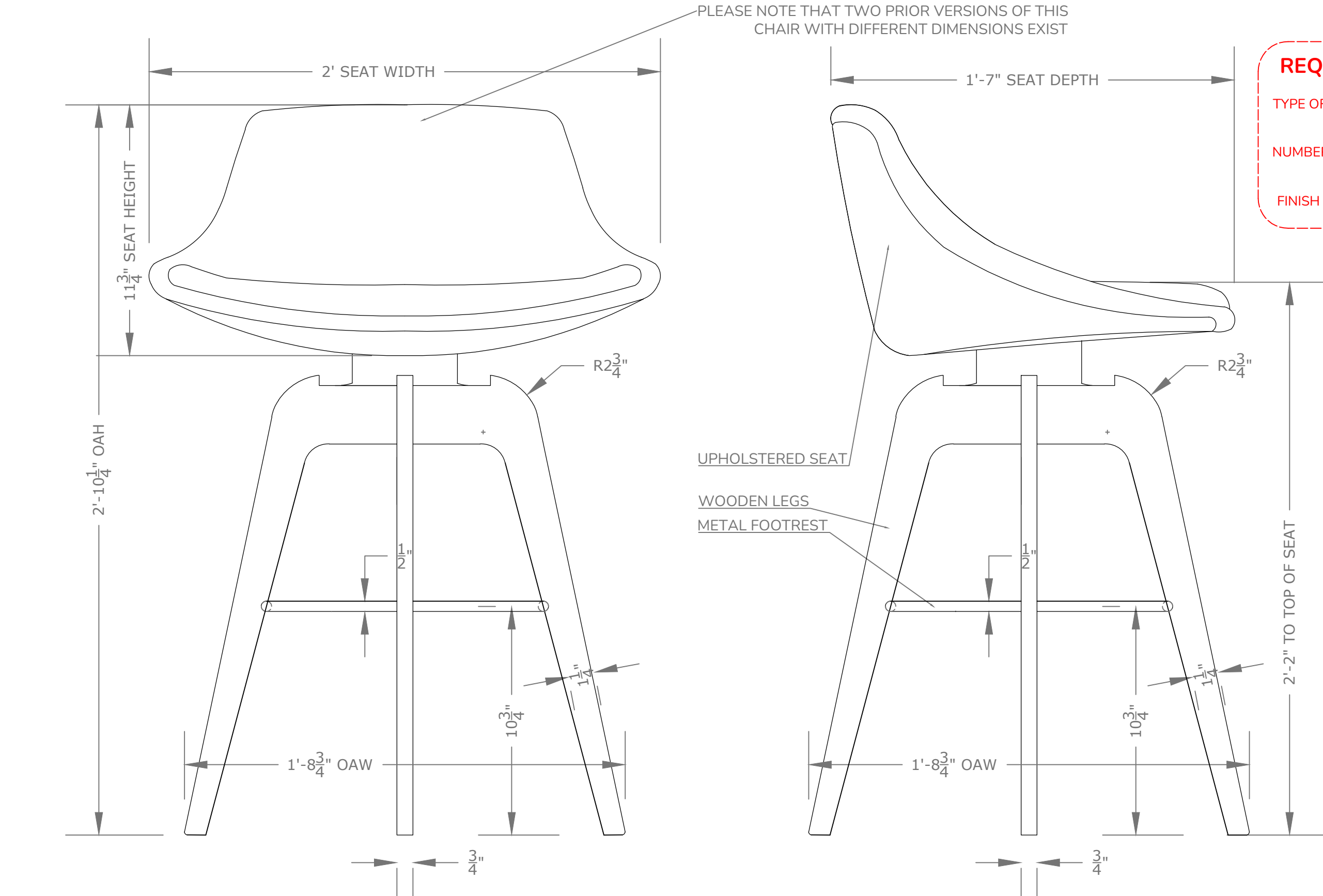
B ELEVATION - FRONT NTS
