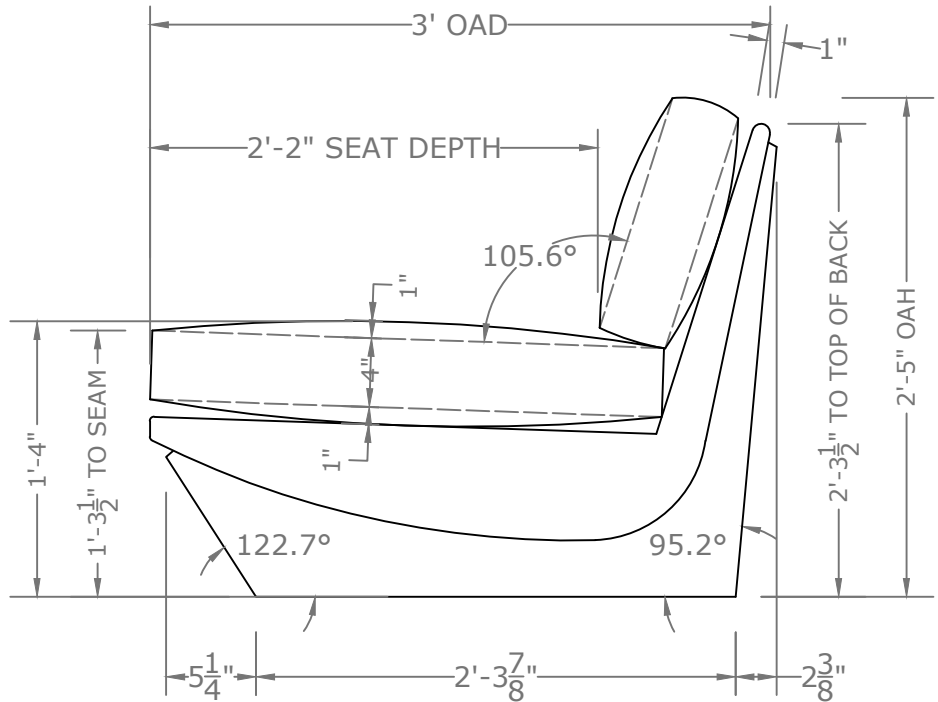
C SECTION A - A - SOFA NTS
