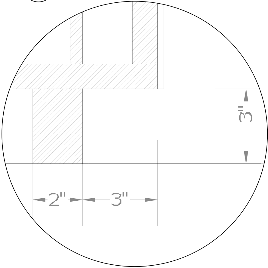
R DETAIL D - TOE KICK AT RECEPTION DESK NTS
