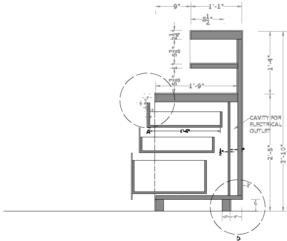
J RECEPTION DESK SECTION F - F NTS
