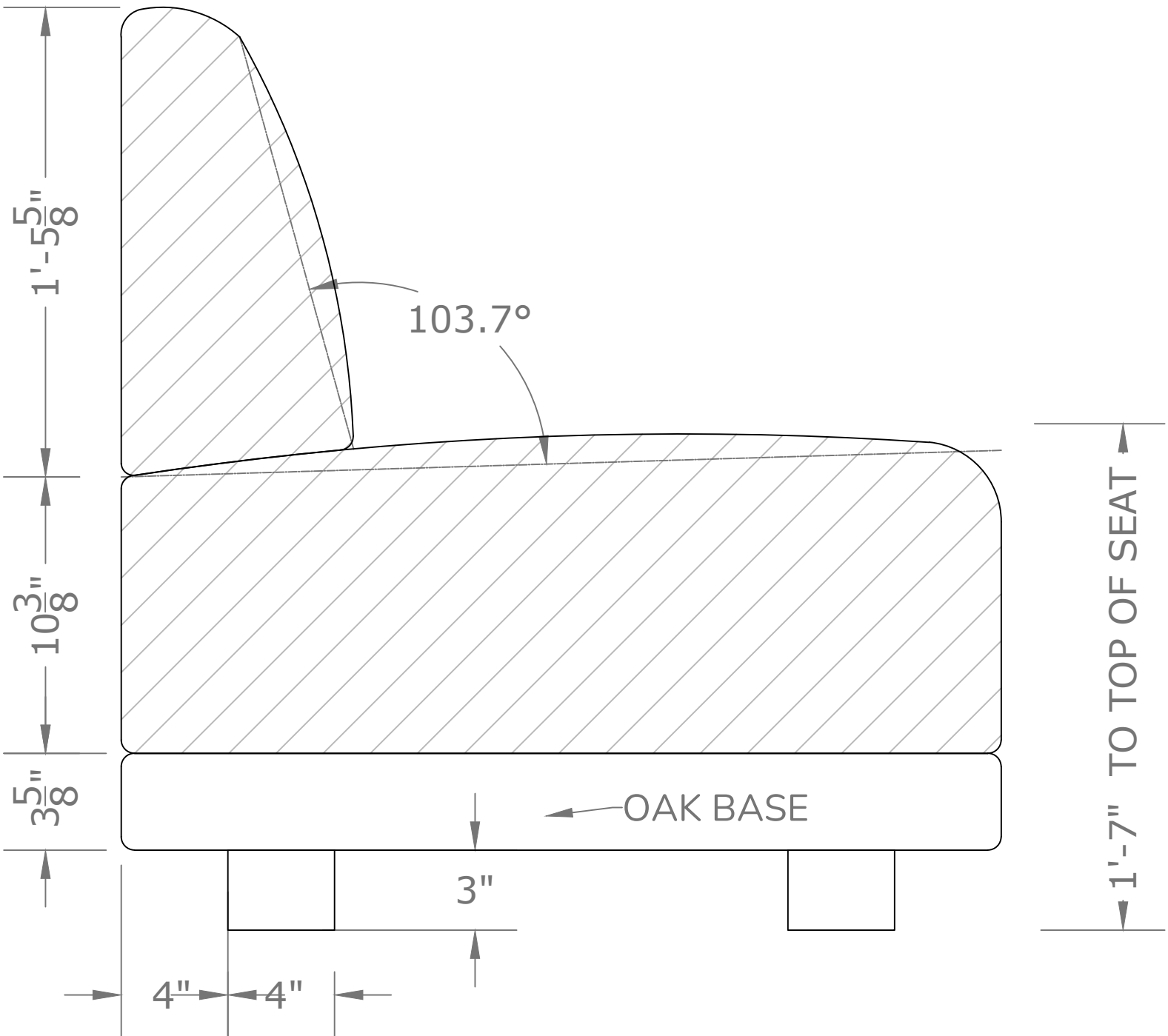
C SECTION A - A NTS
