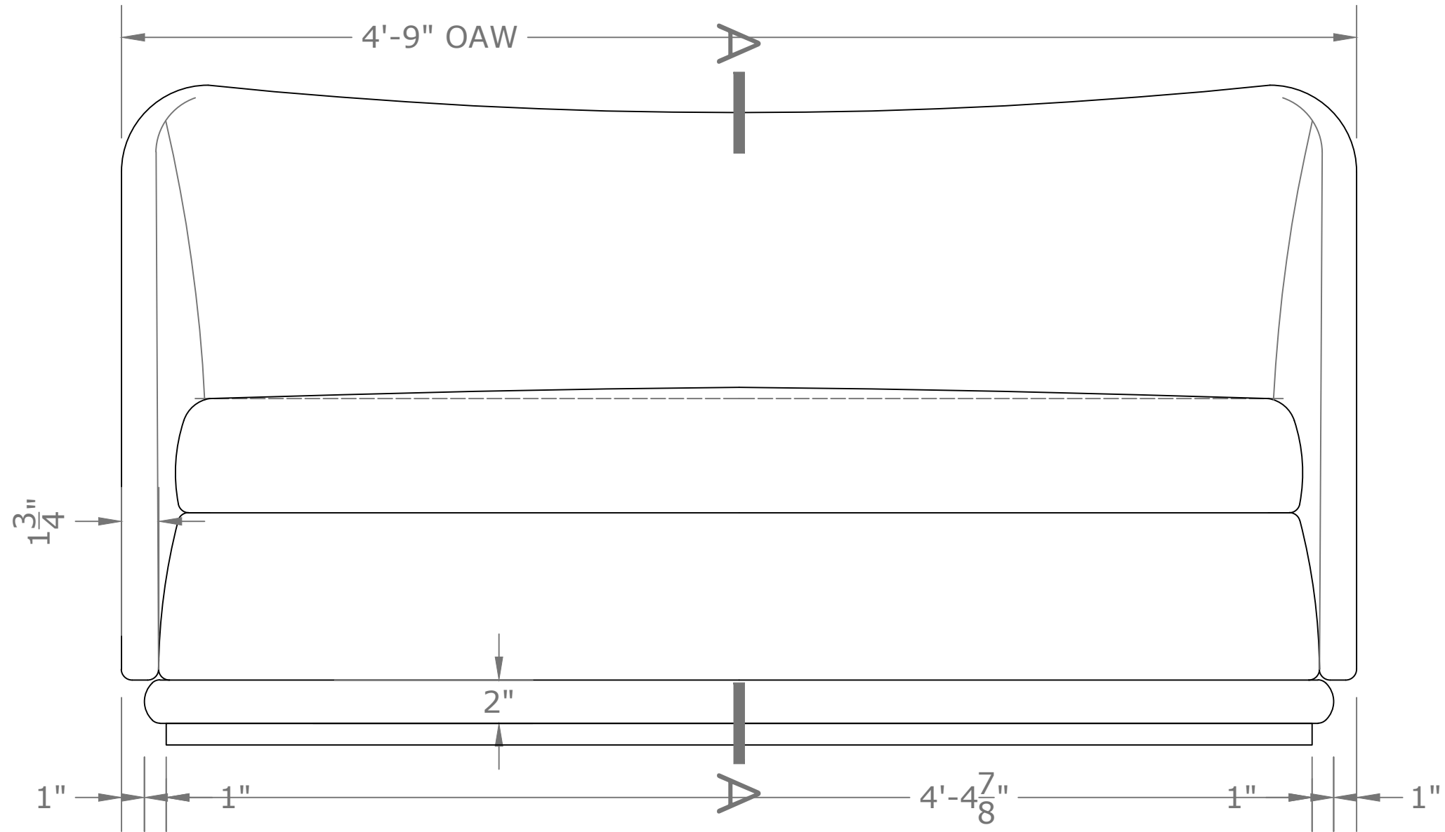
B ELEVATION VIEW - FRONTAL NTS
