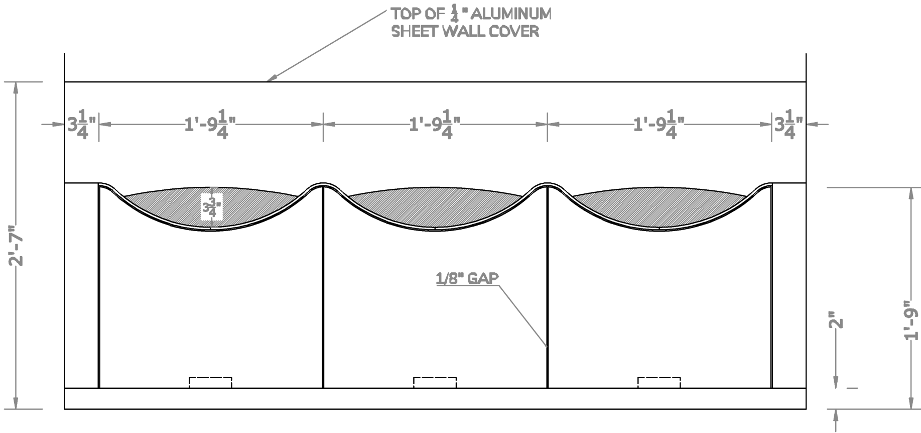
E ELEVATION NTS
