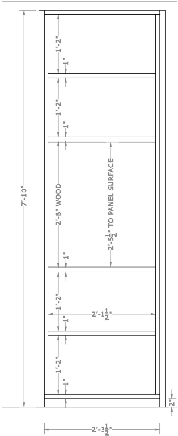
K SHELF SECTION H - H NTS
