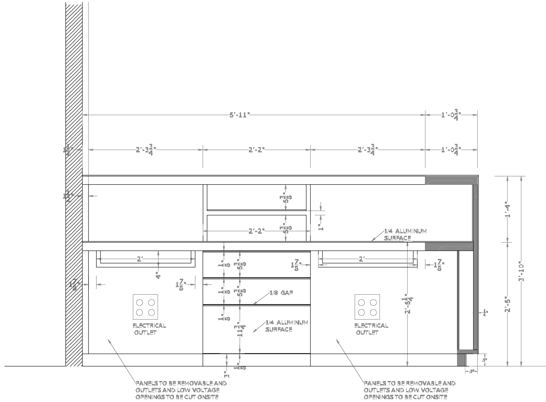
I RECEPTION DESK SECTION E - E NTS
