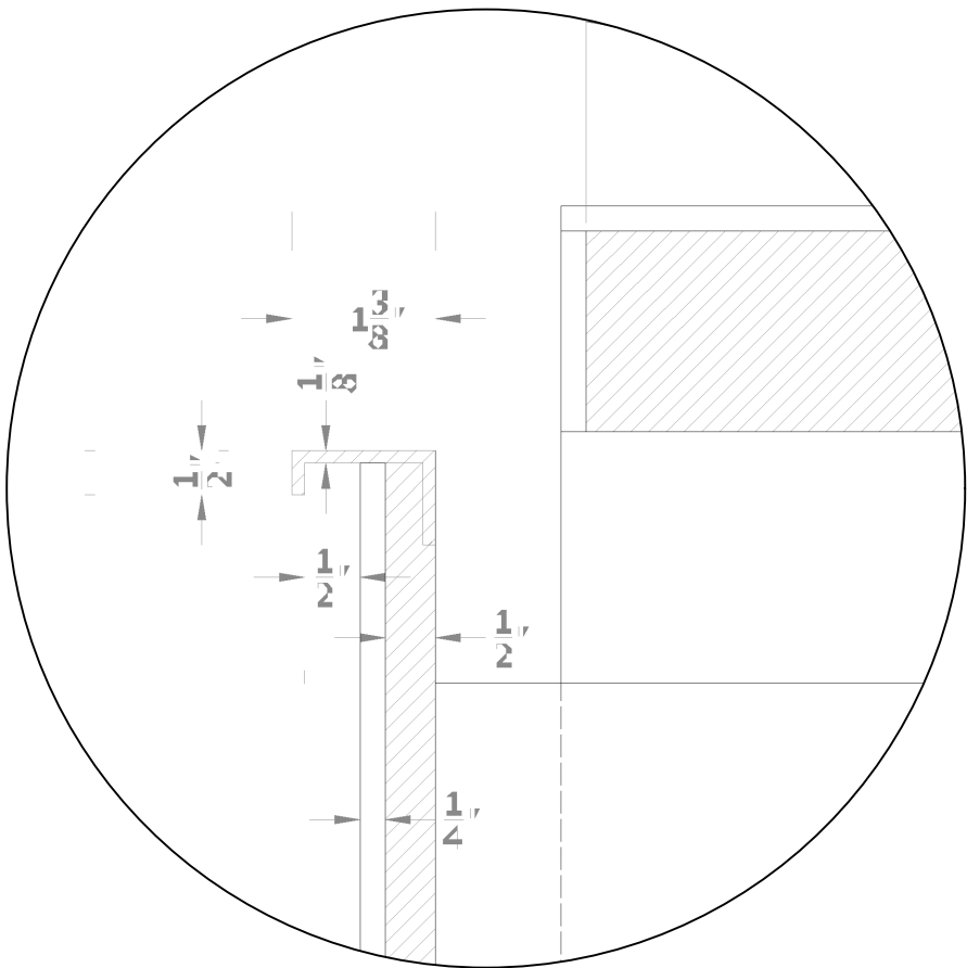
N DETAIL A - PULL ON DRAWER NTS
