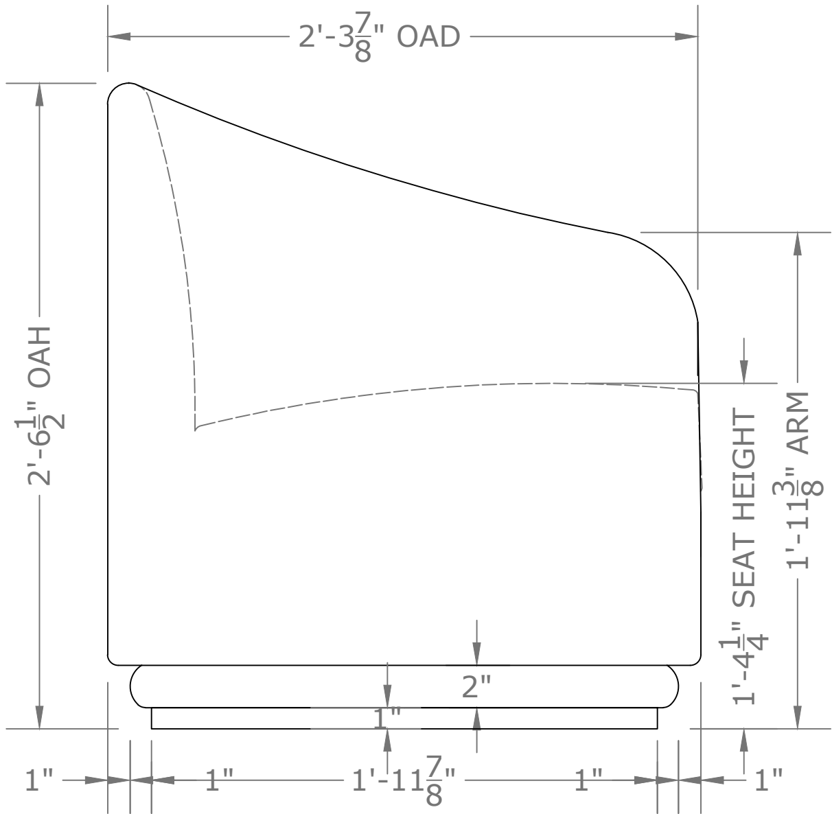
C ELEVATION VIEW - SIDE NTS
