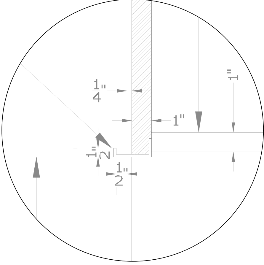
O DETAIL B - PULL ON CABINET DOORS NTS
