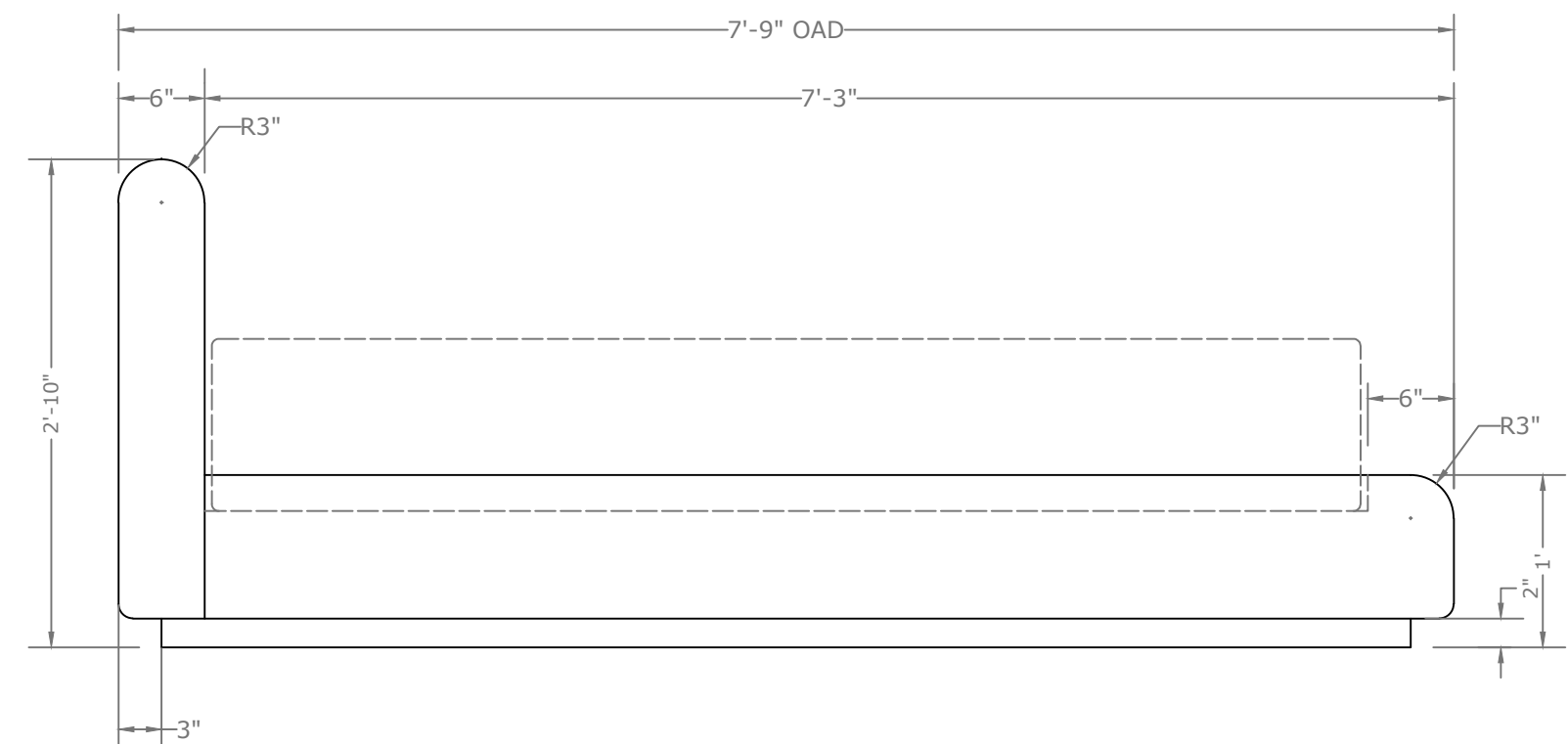
C SIDE VIEW NTS
