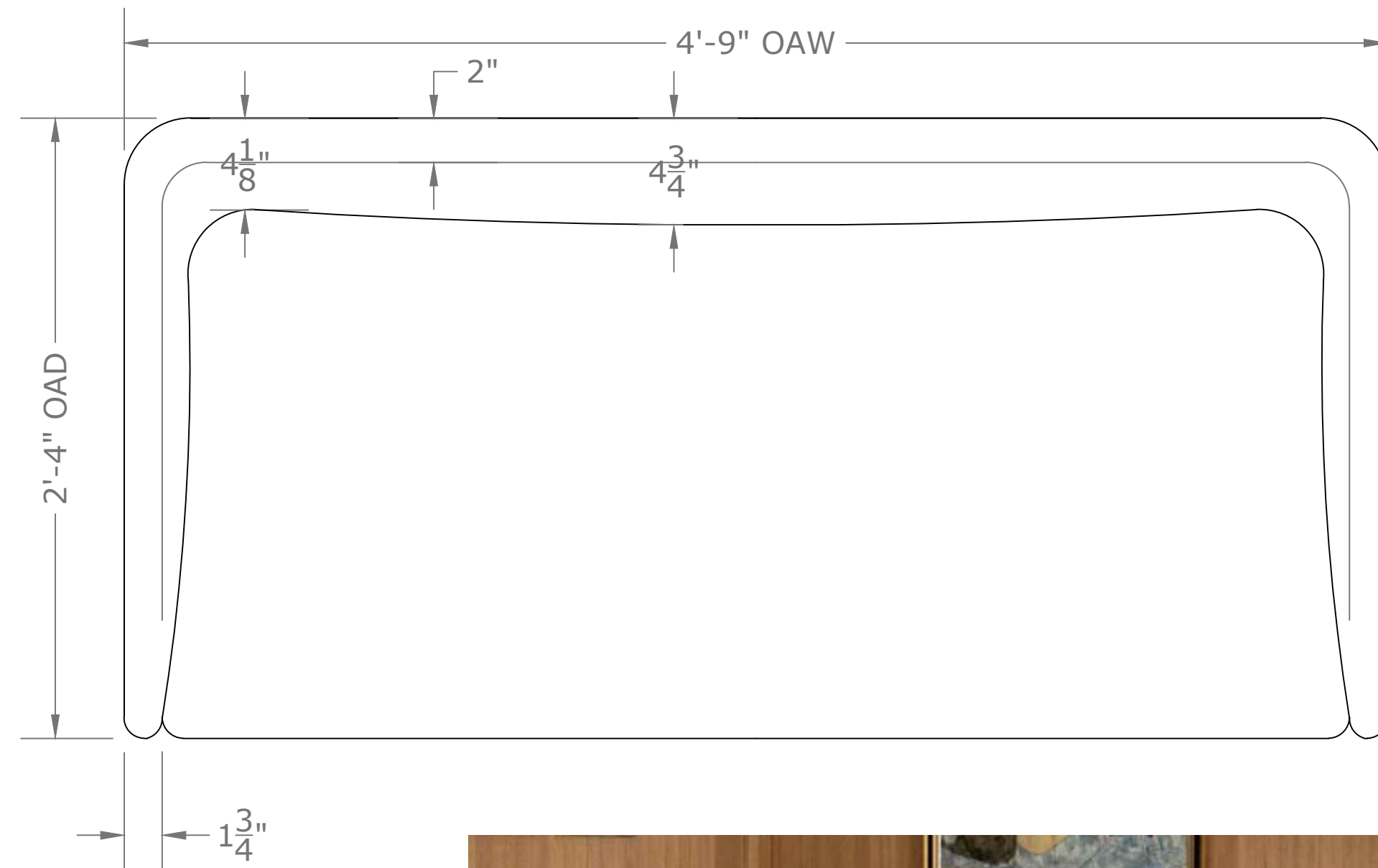
A PLAN VIEW NTS
